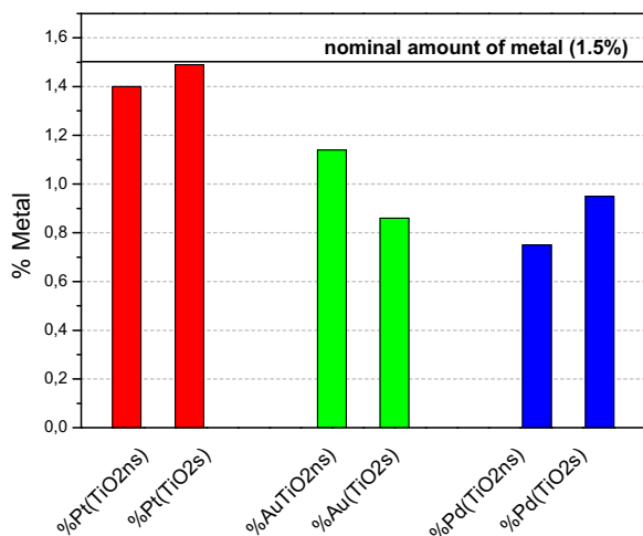
Fig. 5. Total metal content (measured by XRF) for the sulphated and non-sulphated samples in the three systems: Pt/TiO 2 , Au/TiO 2 , Pd/TiO 2 .
