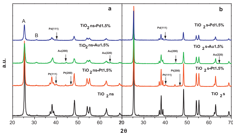
Fig. 1. XRD patterns for (a) non-sulphated and (b) sulphated \text{TiO}_2 , displaying undoped samples and samples with 1.5 wt.% photodeposited Pt, Au, and Pd. A: anatase and B: brookite.
