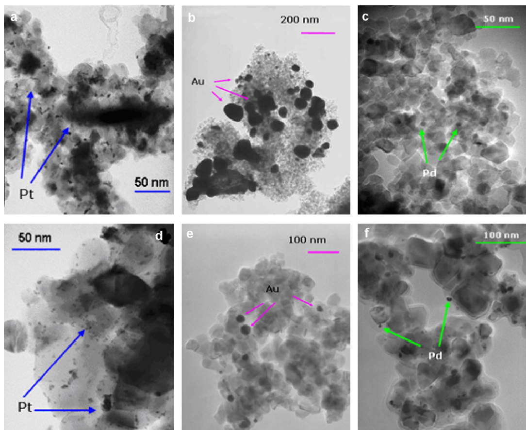
Fig. 3. Selected TEM micrographs for (a) \text{TiO}_2\text{ns-Pt} (b) \text{TiO}_2\text{ns-Au} (c) \text{TiO}_2\text{ns-Pd} (d) \text{TiO}_2\text{s-Pt} , (e) \text{TiO}_2\text{s-Au} and (f) \text{TiO}_2\text{s-Pd} .
