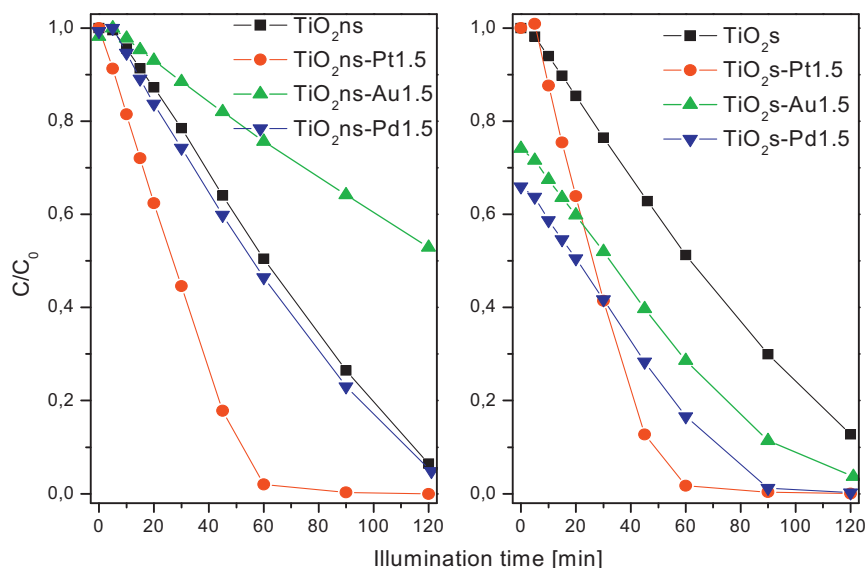
Fig. 7. Profiles of phenol degradation over the different non-sulphated (a) and pre-sulphated photocatalysts (b) with the illumination time. [Phenol] 0 = 50 mg L -1 , V = 0.2 L, [catalyst] = 1 g L -1 , I = 95 W m -2 .
