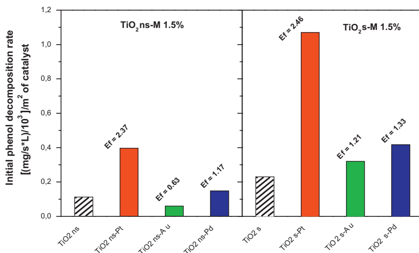
Fig. 8. Initial reaction rates in the decomposition of phenol (mg of phenol degraded per litre per second) normalised per surface area unit of catalyst (m 2 ).
