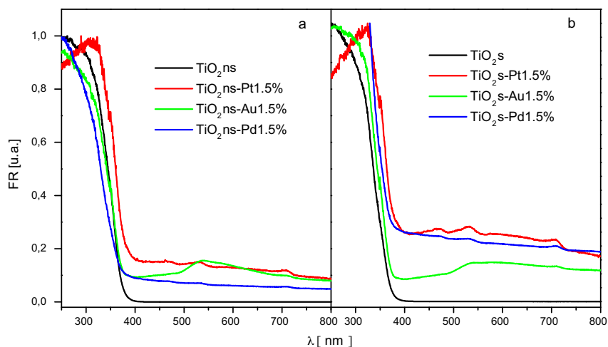
Fig. 2. UV-vis diffuse reflectance spectra for (a) non-sulphated and (b) sulphated \text{TiO}_2 , displaying undoped samples and samples with 1.5 wt.% photodeposited Pt, Au, and Pd.
