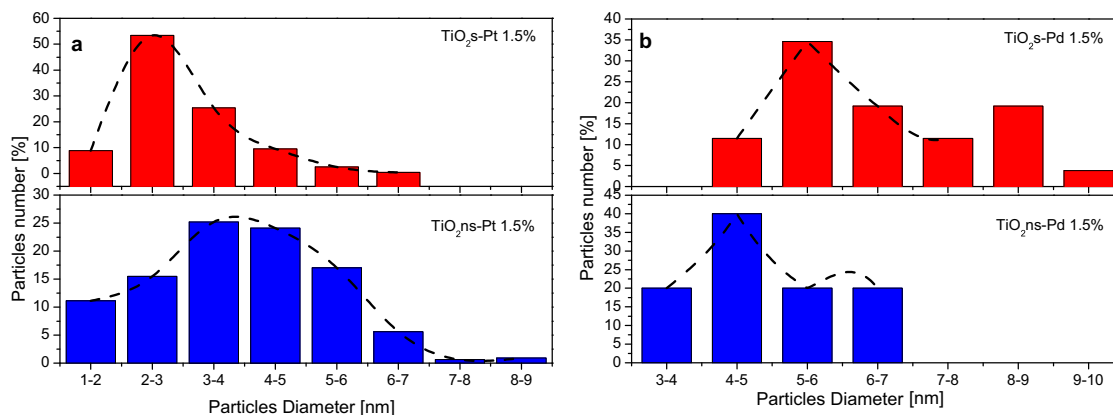
Fig. 4. Particle size distribution for (a) Pt and (b) Pd clusters, determined by counting deposits in a large number of TEM micrographs.
